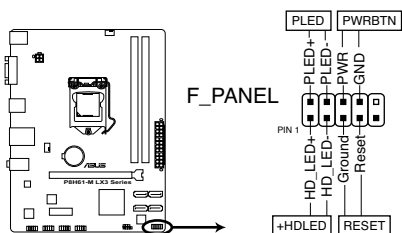
P8H61-M LX3 Series System panel connector
