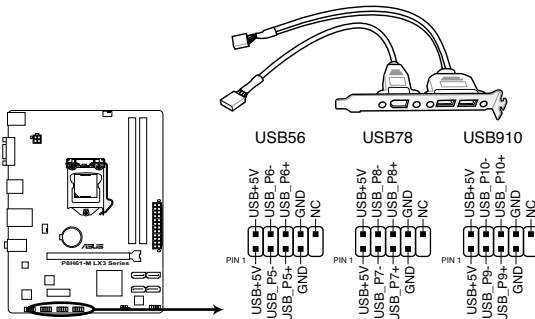
P8H61-M LX3 Series USB2.0 connectors
